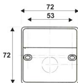
Dimensions & Electrical Connections
