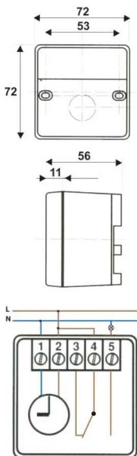
Dimensions & Electrical Connections
